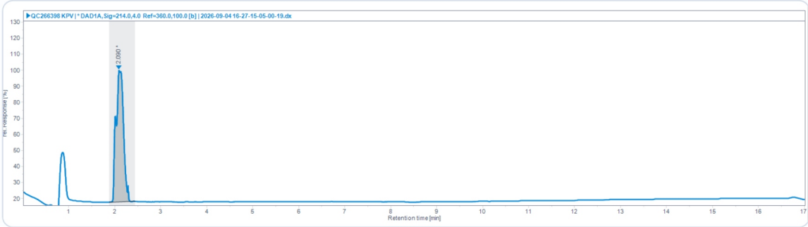
HPLC Chromatogram · Retention Time 2.090 min
