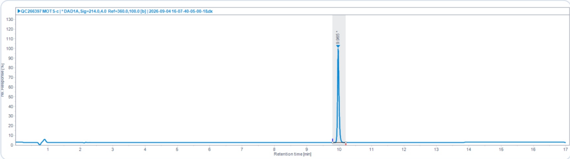
HPLC Chromatogram · Retention Time 9.965 min
