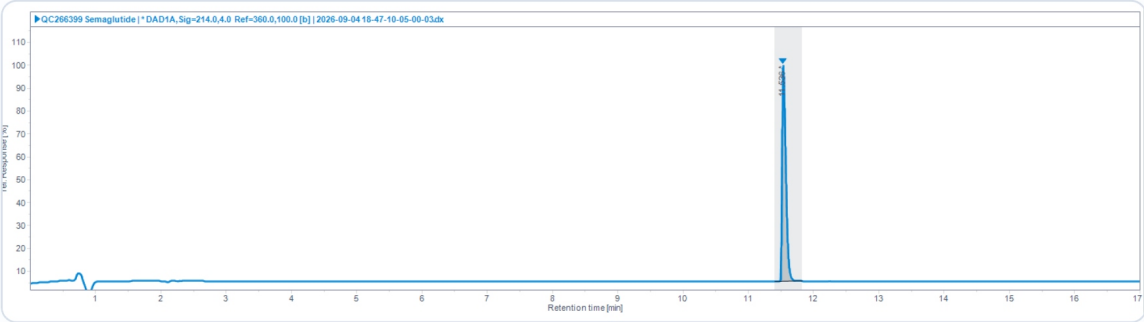
HPLC Chromatogram · Retention Time 11.536 min
